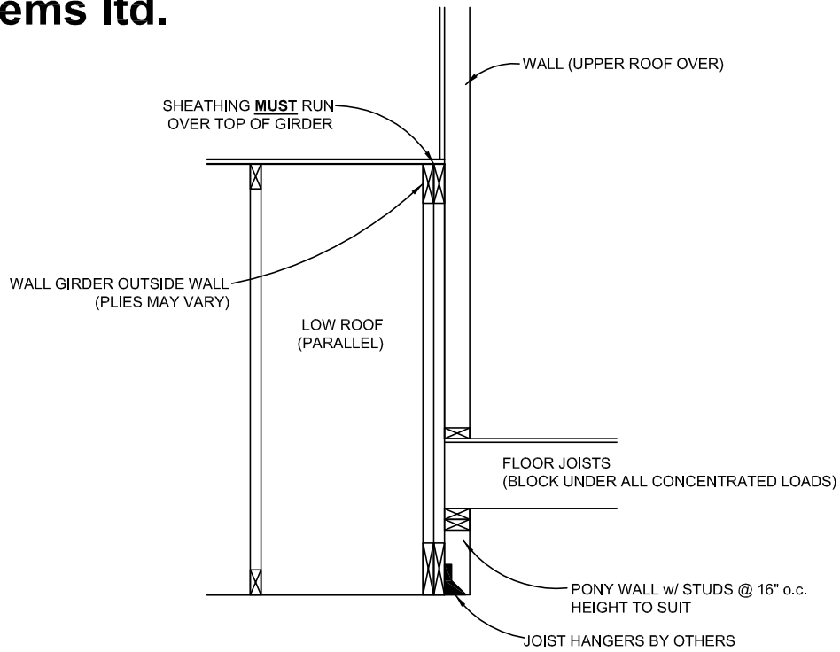
J WALL GIRDER OUTSIDE, ROOF PARALLEL WITH PONY WALL NOT TO SCALE
