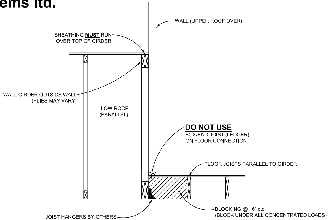
G WALL GIRDER OUTSIDE, ROOF PARALLEL, FLOOR PARALLEL NOT TO SCALE
