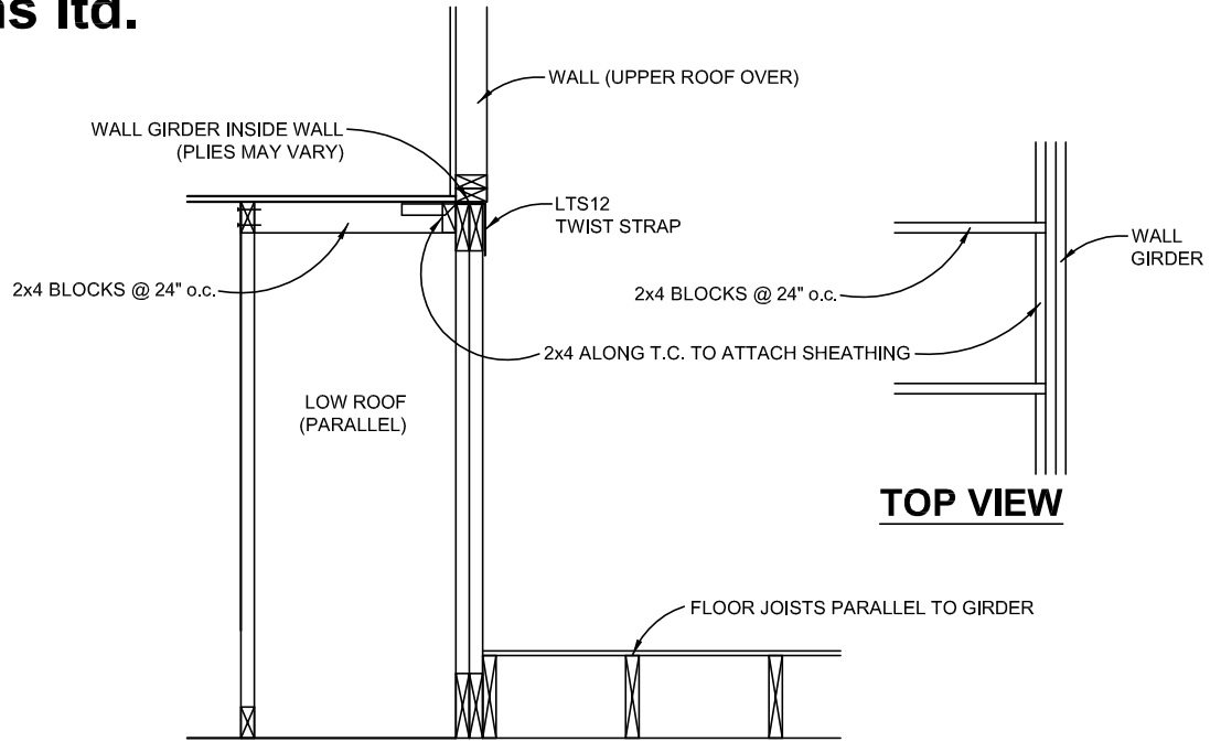
C WALL GIRDER INSIDE, ROOF PARALLEL, FLOOR PARALLEL NOT TO SCALE
