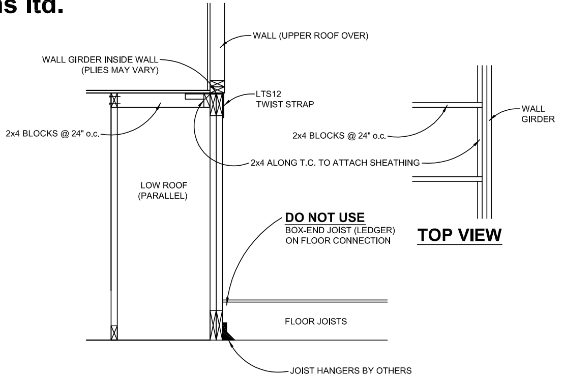
A WALL GIRDER INSIDE, ROOF PARALLEL, FLOOR PERPENDICULAR NOT TO SCALE
