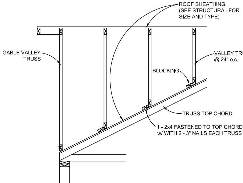
VALLEY AT GABLE END
